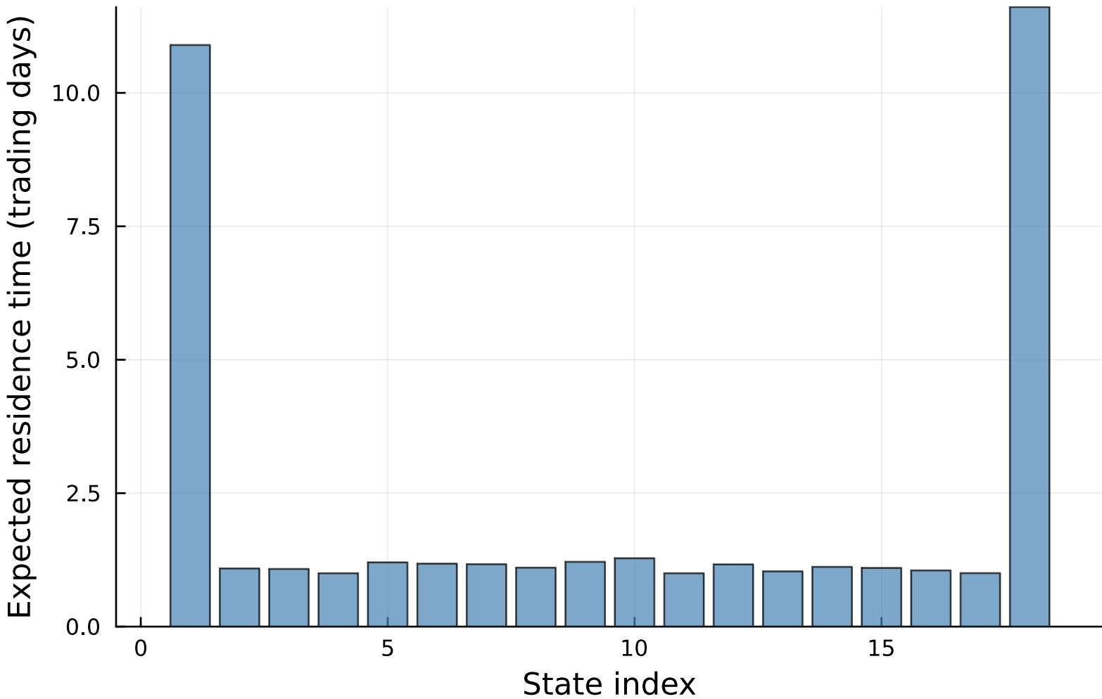
Natural residence time 1/(1 - T_{ii}) | SPY | CHMM-N, K=18
