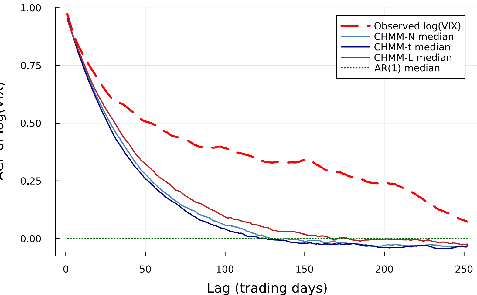
(c) ACF(log VIX), lag 1..252
