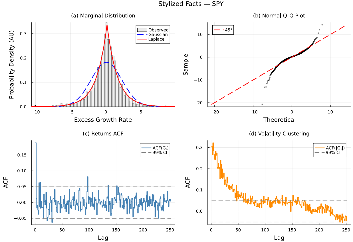
Figure 9. Empirical stylized facts of SPY daily excess growth rates (IS, 2014-01-03 through 2024-01-03). Panel (a): leptokurtic marginal distribution with Gaussian and Laplace fits. Panel (b): normal Q-Q plot confirming heavy tails. Panel (c): near-zero autocorrelation of raw returns. Panel (d): persistent autocorrelation of absolute returns characterizing volatility clustering.
