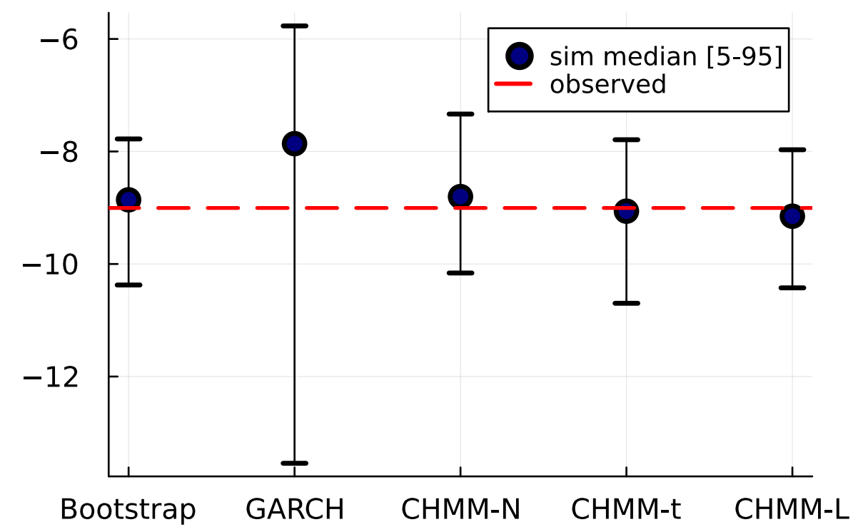
IS ES (0.01)
