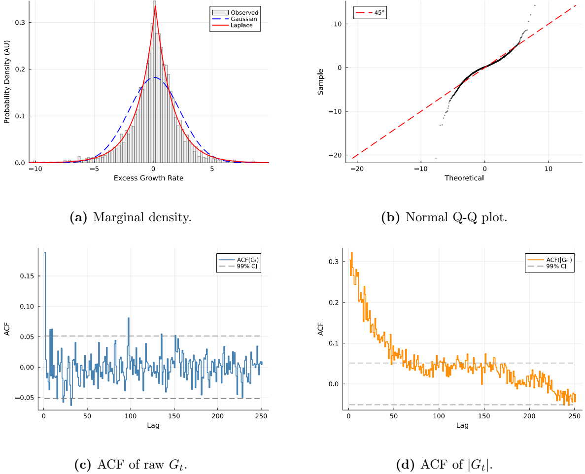
Figure 4. The three Cont stylized facts on SPY IS. (a) marginal density with maximum-likelihood Gaussian and Laplace overlays; (b) normal Q-Q plot; (c) empirical ACF of raw G_t at lags 1–252 with 99% Bartlett band; (d) empirical ACF of |G_t| on the same window.
