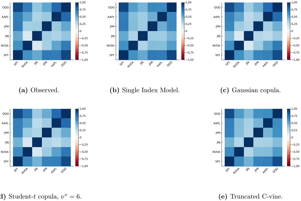
Figure 36. Cross-asset IS correlation reproduction across dependence models (Pipeline B, companion to Table 67). Panel (a): observed correlation matrix on 2014-01-03 through 2024-01-03 daily excess log returns for SPY, NVDA, JNJ, JPM, AAPL, QQQ (IS window, T_{IS} = 2,516 ). Panel (b): path-averaged correlation under the Single Index Model with SPY as market factor. Panel (c): path-averaged correlation under the Gaussian copula on CHMM marginals. Panel (d): path-averaged correlation under the Student- t copula on CHMM marginals, \nu^* = 6 . Panel (e): path-averaged correlation under a truncated C-vine copula with SPY as root. Each simulated panel averages over 200 paths of length T_{IS} . All marginals are the per-asset CHMM-N fits at K = 18 from Table 7; color scale in [-1, 1] , red-white-blue (RdBu) diverging. Closer visual match to panel (a) is better.
