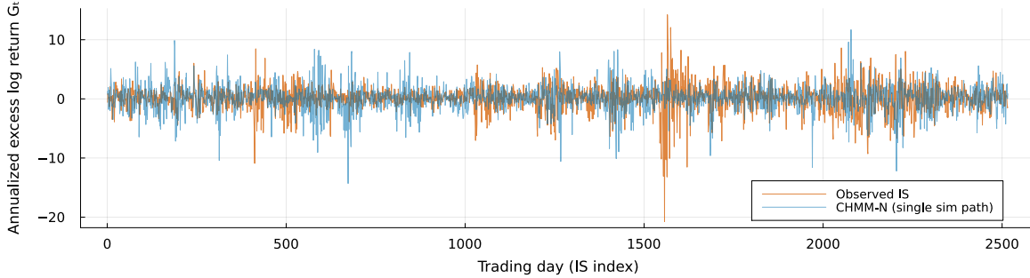
(a) In-sample window, full T_{IS} = 2,516 trading days.
