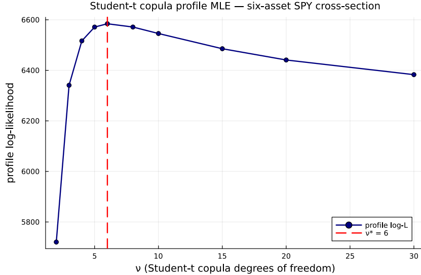
Figure 26: Profile log-likelihood of the Student-t copula on the six-asset SPY cross-section. The dashed red line marks the profile MLE \nu^* = 6 .
