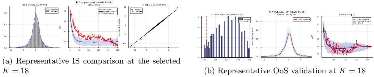
Figure 4: State-resolution summary at the selected operating point K = 18 . The full sweep over K \in \{3, 6, 9, 12, 15, 18, 21\} and per- K figures are reproduced in Appendix A (Table 8 and Figures 14–15).
