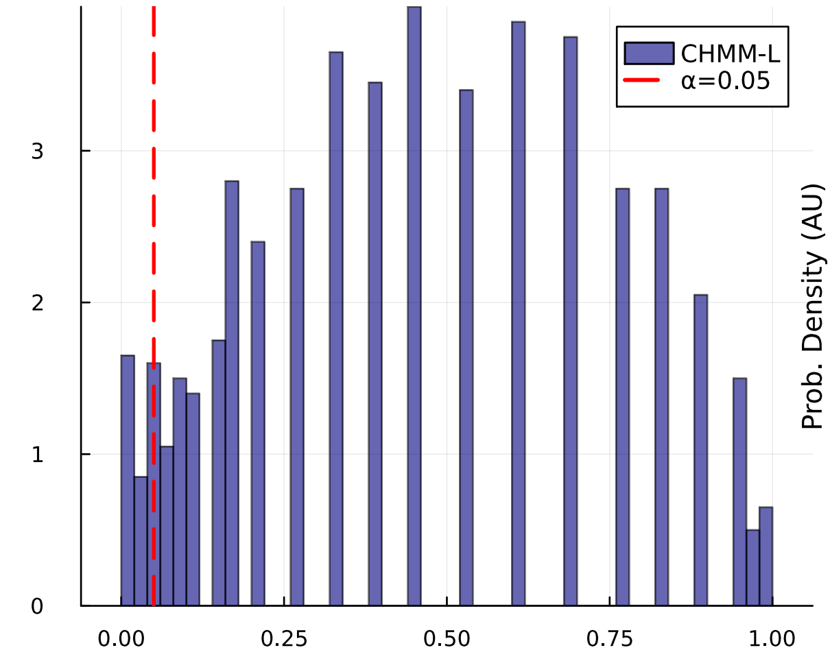
(a) OoS KS p-values (pass: 94.0%)
