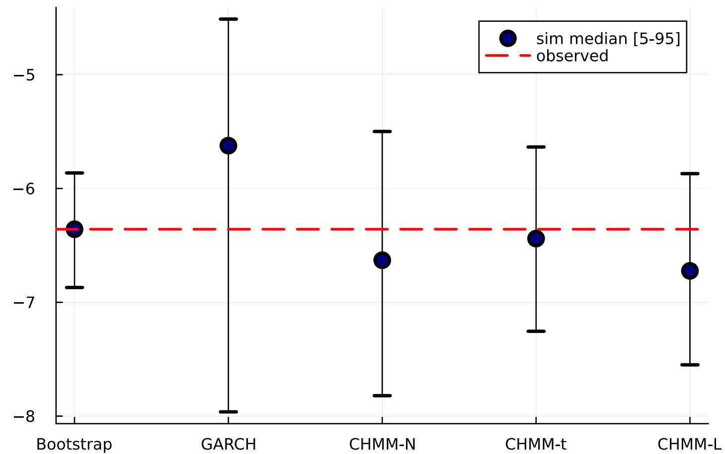
OoS VaR (0.05)
