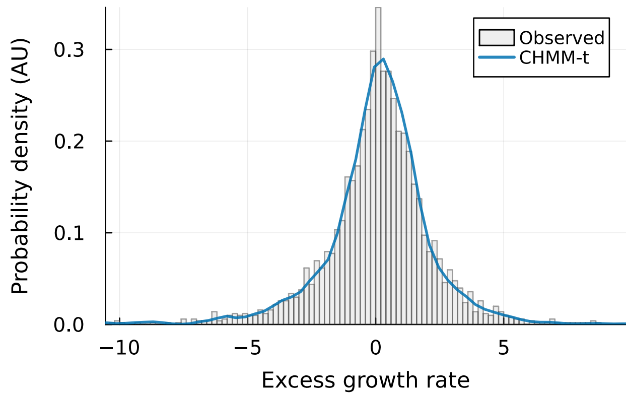
(a) IS density (KS: 95.7%)
