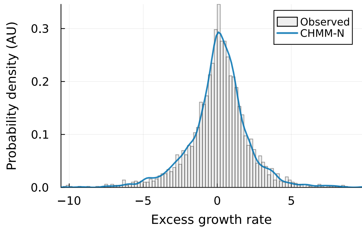
(a) IS density (KS: 94.1%)
