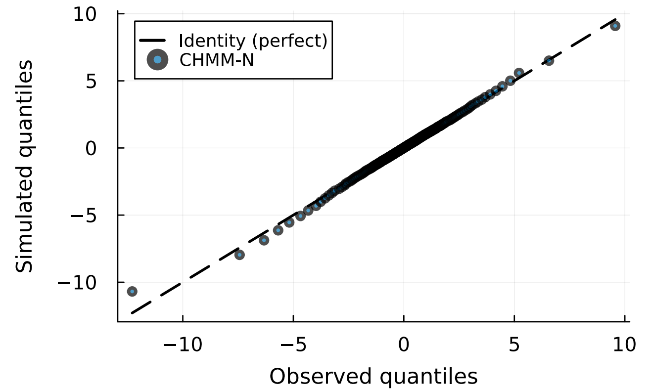
(b) Tail Q-Q plot (0.1st-99.9th)
