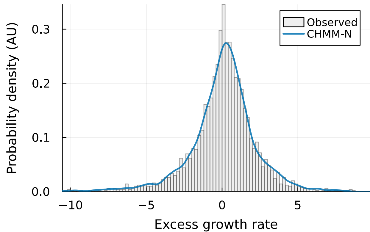
(a) IS density (KS: 95.6%)
