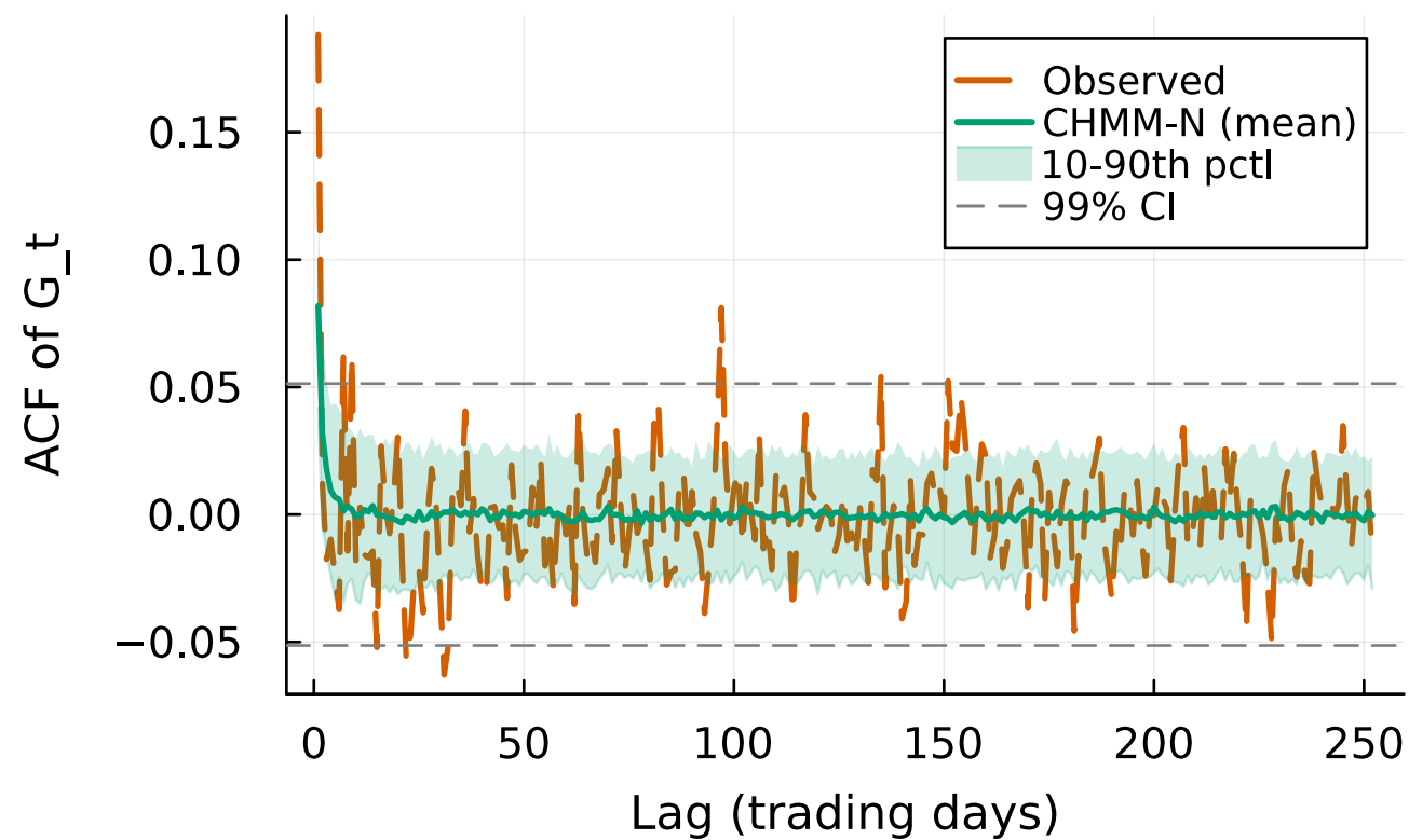
(c) ACF of G_t (raw returns)
