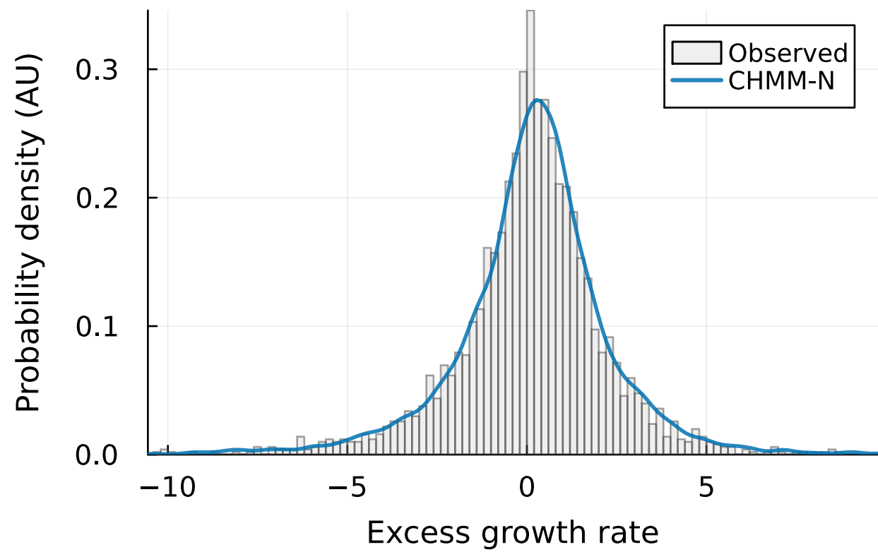
(a) IS density (KS: 90.1%)
