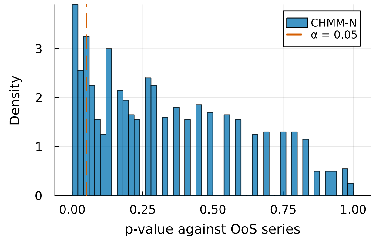
(b) OoS KS p-values (pass: 83.2%)
