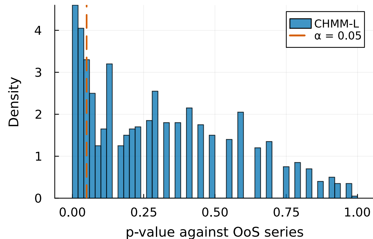
(b) OoS KS p-values (pass: 77.9%)
