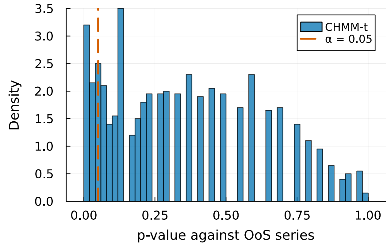
(b) OoS KS p-values (pass: 86.2%)
