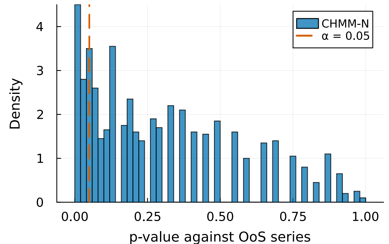
(b) OoS KS p-values (pass: 79.7%)
