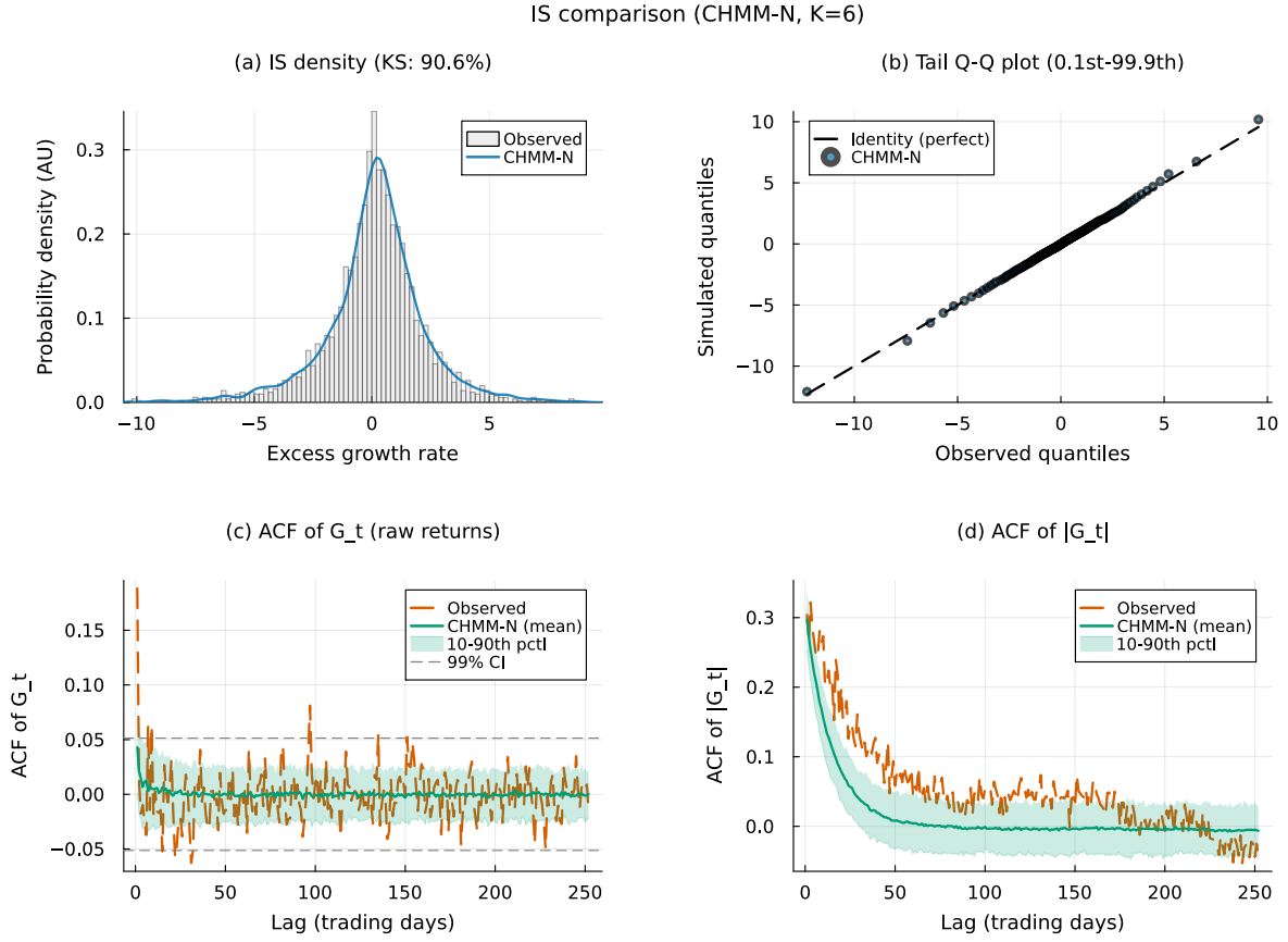
Figure 10. IS SPY CHMM-N comparison at K = 6 (Pipeline A, 1,000 simulated paths; panels as in Figure 4).
