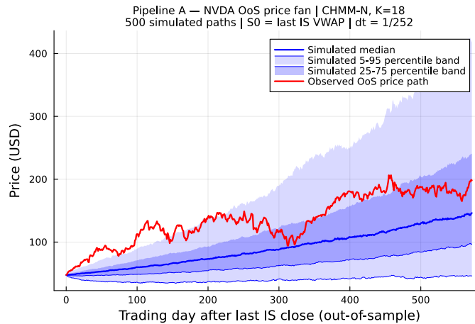
Figure 24. NVDA OoS price fan, CHMM-N ( S_0 = 47.67 \rightarrow P_T^{\text{obs}} = 198.07 , a 4.15\times rally). The observed path exits the 25–75% interquartile band by mid-horizon but remains inside the 5–95% envelope; horizon-wide coverage under CHMM-N is 0.70 (CHMM-t: 0.64, CHMM-L: 0.67; Table 14), the lone calibration outlier in the panel.
