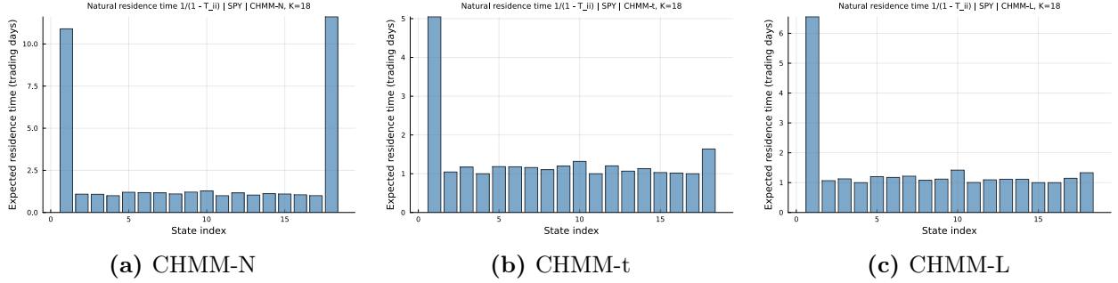
Figure 18. Natural residence times \tau_k = 1/(1 - T_{kk}) at K = 18 for the SPY IS fit (Pipeline A) across the three emission families (CHMM-N Gaussian, CHMM-t Student-t, CHMM-L Laplace).
