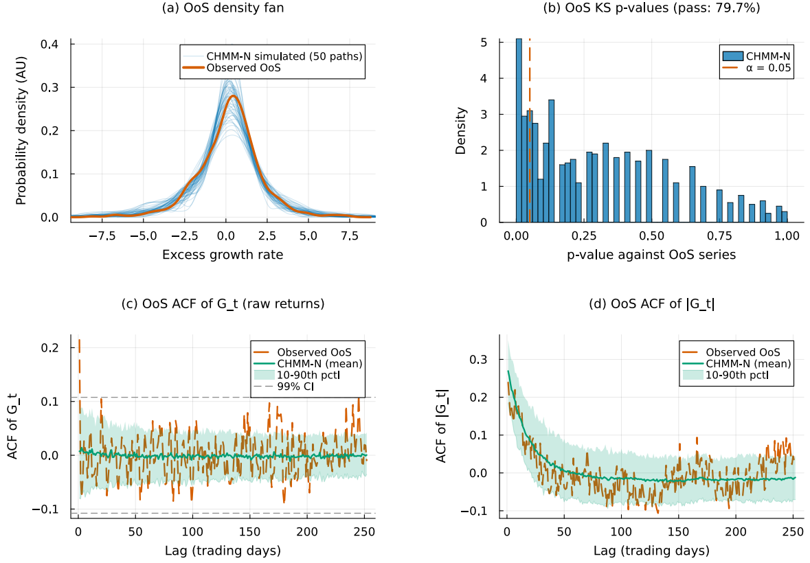
Figure 13. OoS SPY CHMM-N validation at K = 3 (Pipeline A, 1,000 simulated paths; panels as in Figure 5). The K = 18 counterpart is Figure 5 of the main text.
