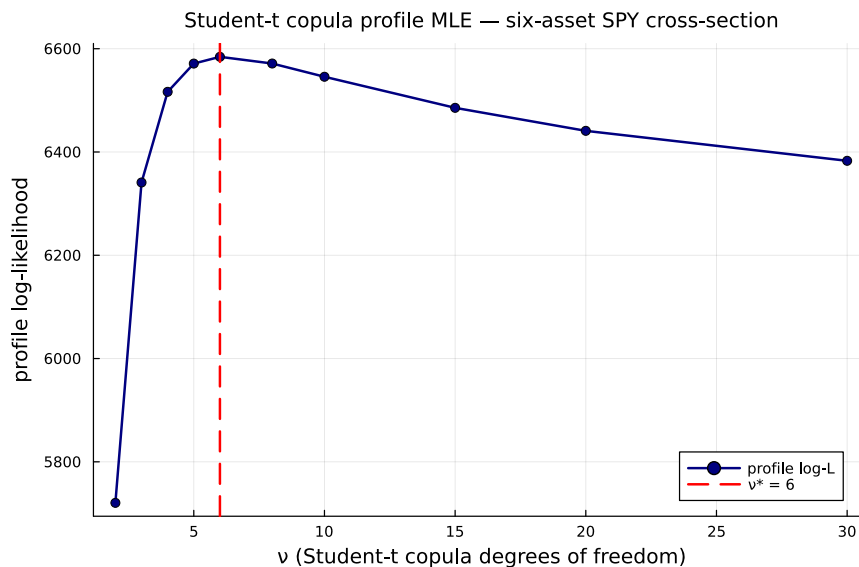
Figure 30. Profile log-likelihood of the Student-t copula used inside Pipeline B on the six-asset SPY cross-section (SPY, NVDA, JNJ, JPM, AAPL, QQQ; IS window 2014-01-03 through 2024-01-03). The vertical axis is the profile log-likelihood evaluated at each degrees-of-freedom value \nu on the grid \{2, 3, 4, 5, 6, 8, 10, 15, 20, 30\} ; the dashed red line marks the profile MLE \nu^* = 6 (peak value 6157.47). The CHMM-N marginals are held fixed at the Pipeline A per-asset fits while \nu is varied.
