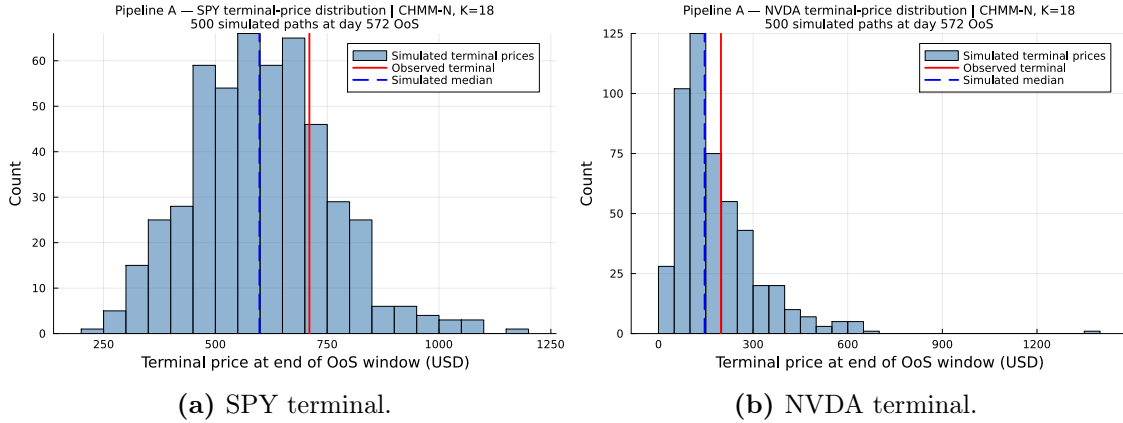
Figure 25. OoS terminal-price distributions under CHMM-N for SPY and NVDA. The right-skew is characteristic of log-returns aggregated to prices; the SPY terminal sits close to the simulated median, while the NVDA terminal sits in the upper-right of the simulated distribution (the realised rally is in the upper tail of the CHMM-N terminal density).
