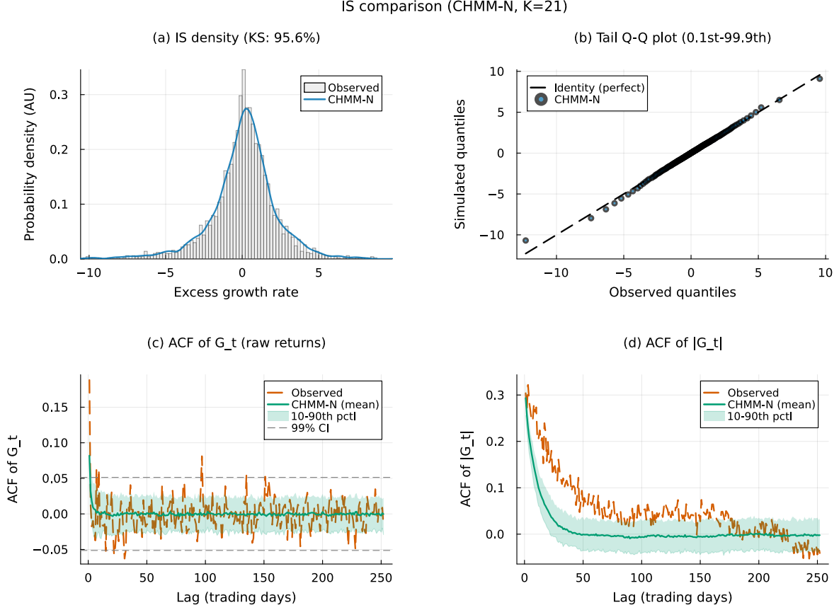
Figure 12. IS SPY CHMM-N comparison at K = 21 (Pipeline A, 1,000 simulated paths; panels as in Figure 4).
