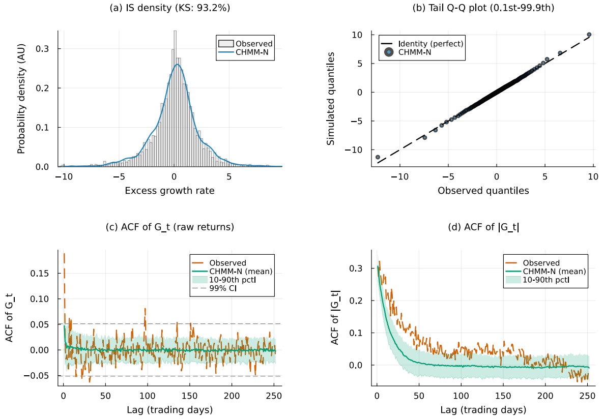
Figure 11. IS SPY CHMM-N comparison at K = 12 (Pipeline A, 1,000 simulated paths; panels as in Figure 4).
