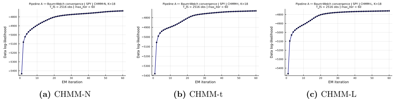
Figure 23. Log-likelihood histories for the SPY IS fit (Pipeline A) at K = 18 across the three emission families (CHMM-N Gaussian classical EM; CHMM-t Student-t ECM with per-state \nu_k golden-section sub-step; CHMM-L Laplace weighted-EM). All three curves are monotonically non-decreasing and plateau well before the max_iter = 60 budget.
