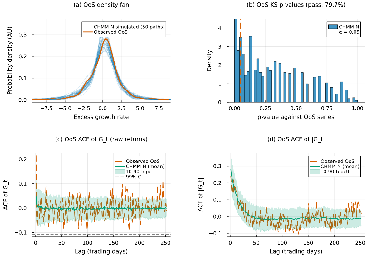
Figure 14. OoS SPY CHMM-N validation at K = 6 (Pipeline A, 1,000 simulated paths; panels as in Figure 5).
