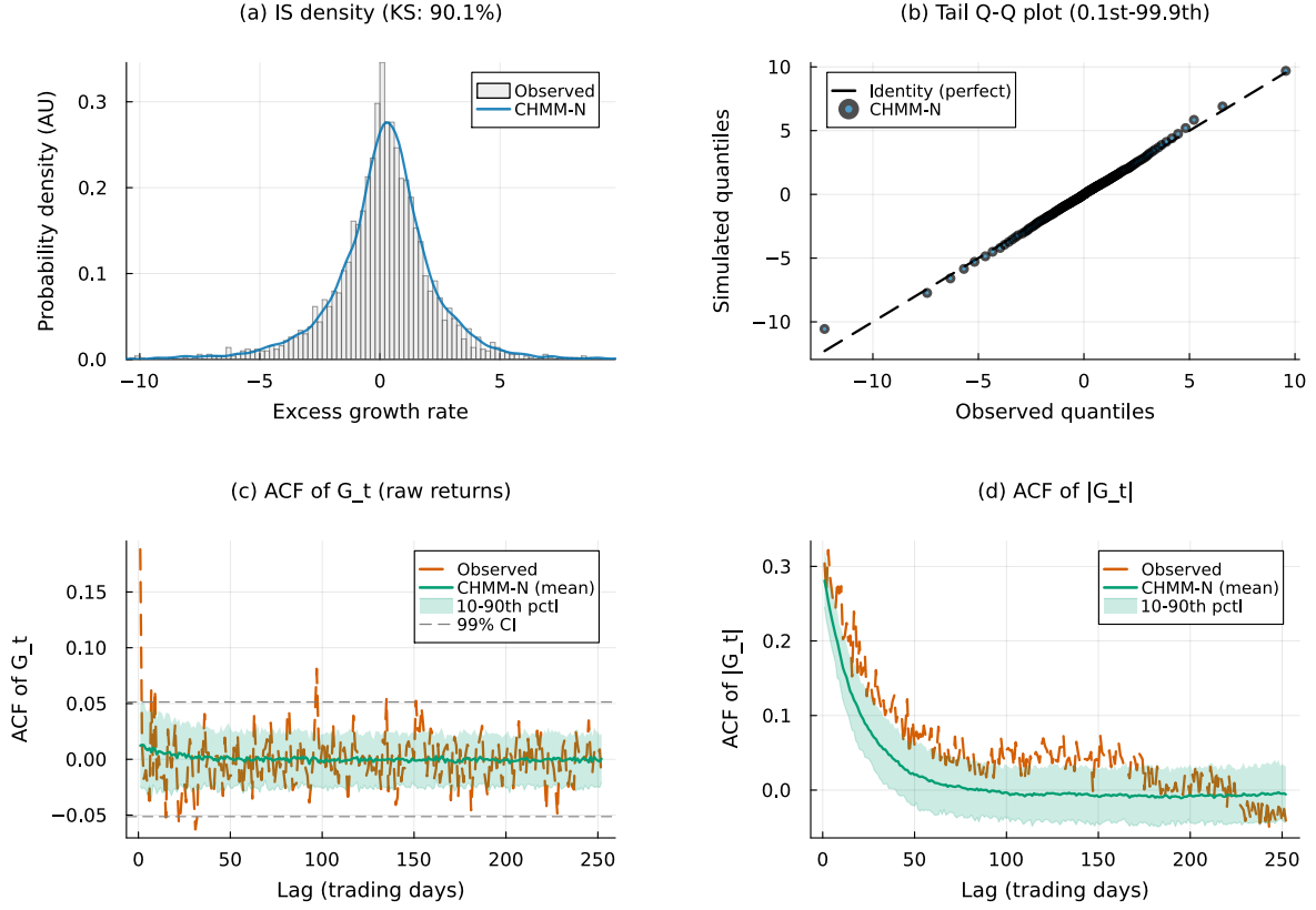
Figure 9. IS SPY CHMM-N comparison at K = 3 (Pipeline A, 1,000 simulated paths; panels as in Figure 4). The K = 18 counterpart is Figure 4 of the main text.
