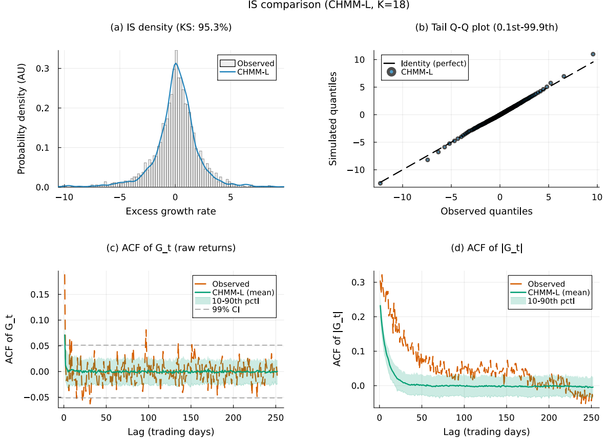
Figure 20. IS SPY model comparison at K = 18 for CHMM-L Laplace emissions (Pipeline A, 1,000 simulated paths). Panels as in Figure 19.
