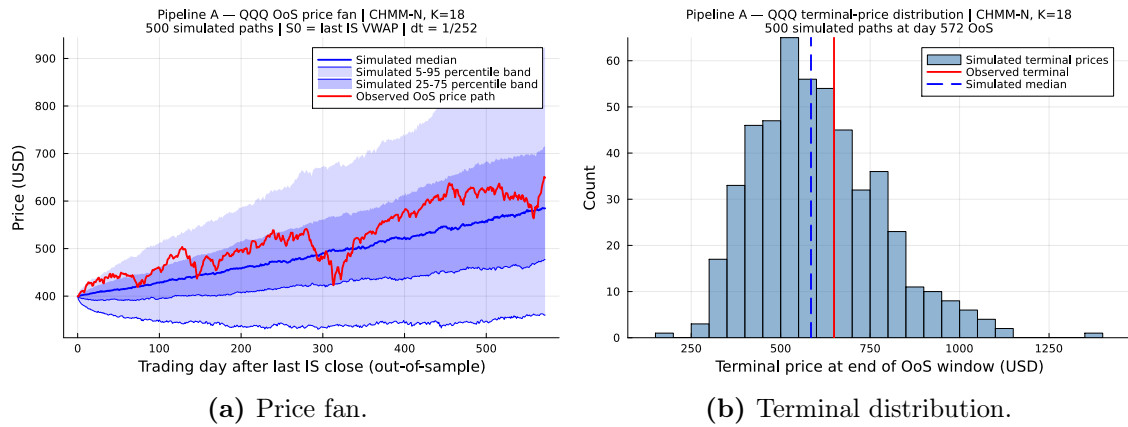
Figure 29. QQQ OoS price fan and terminal distribution, CHMM-N (Pipeline A, K = 18 , 500 simulated paths, T_{\text{OoS}} = 572 ; plotting conventions as above).
