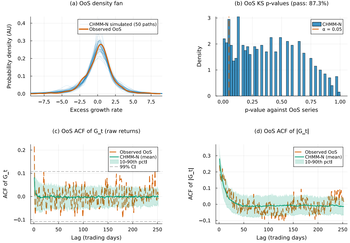
OoS validation (CHMM-N, K=21 )
