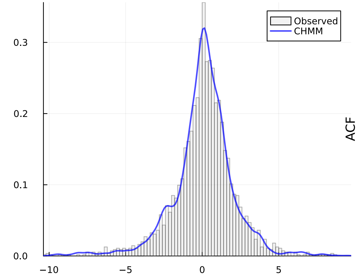
(a) Density (KS pass: 93.6%)
