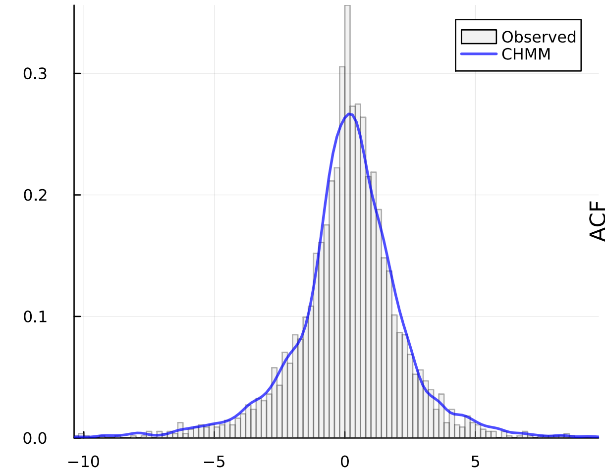
(a) Density (KS pass: 91.8%)
