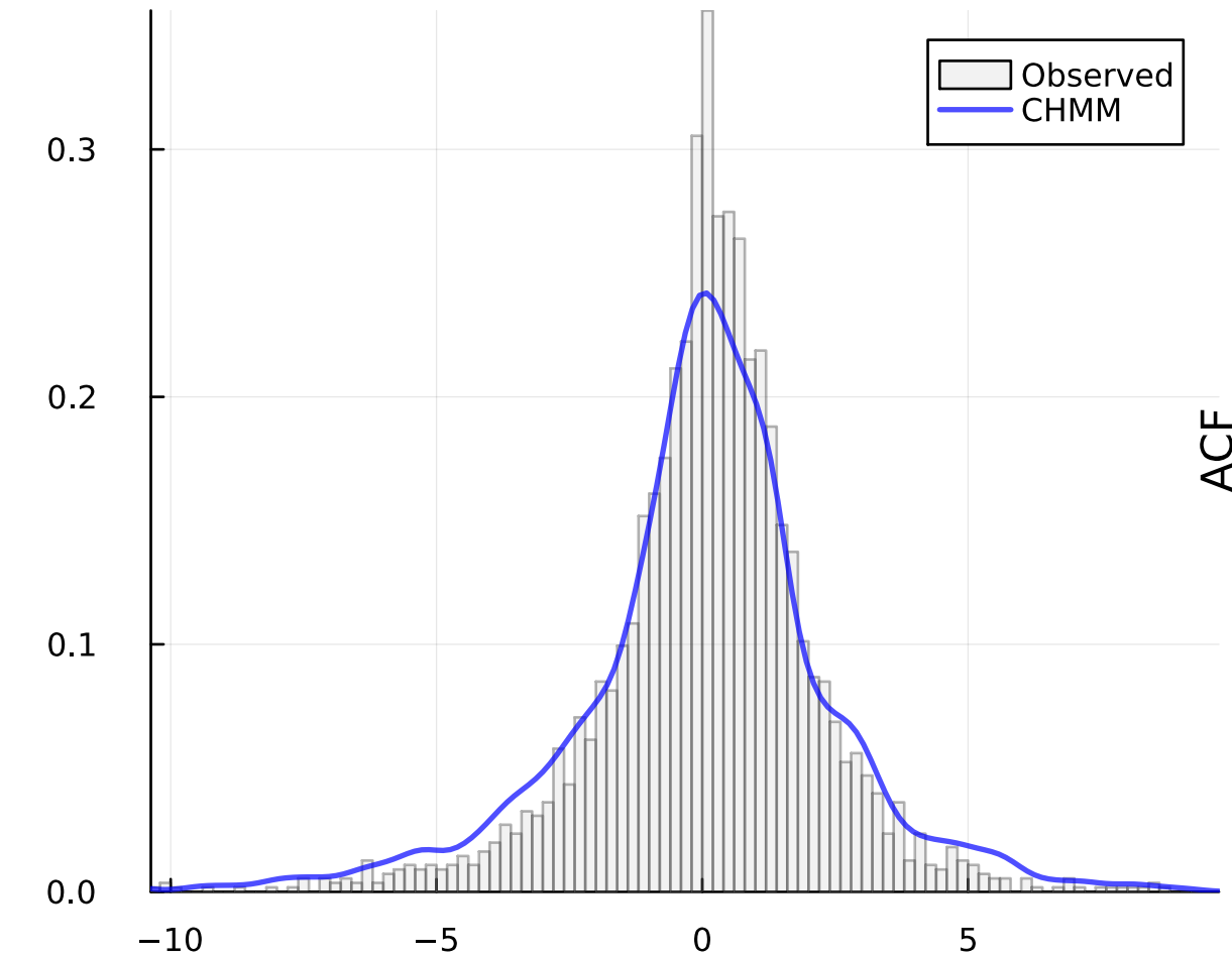
(a) Density (KS pass: 90.8%)
