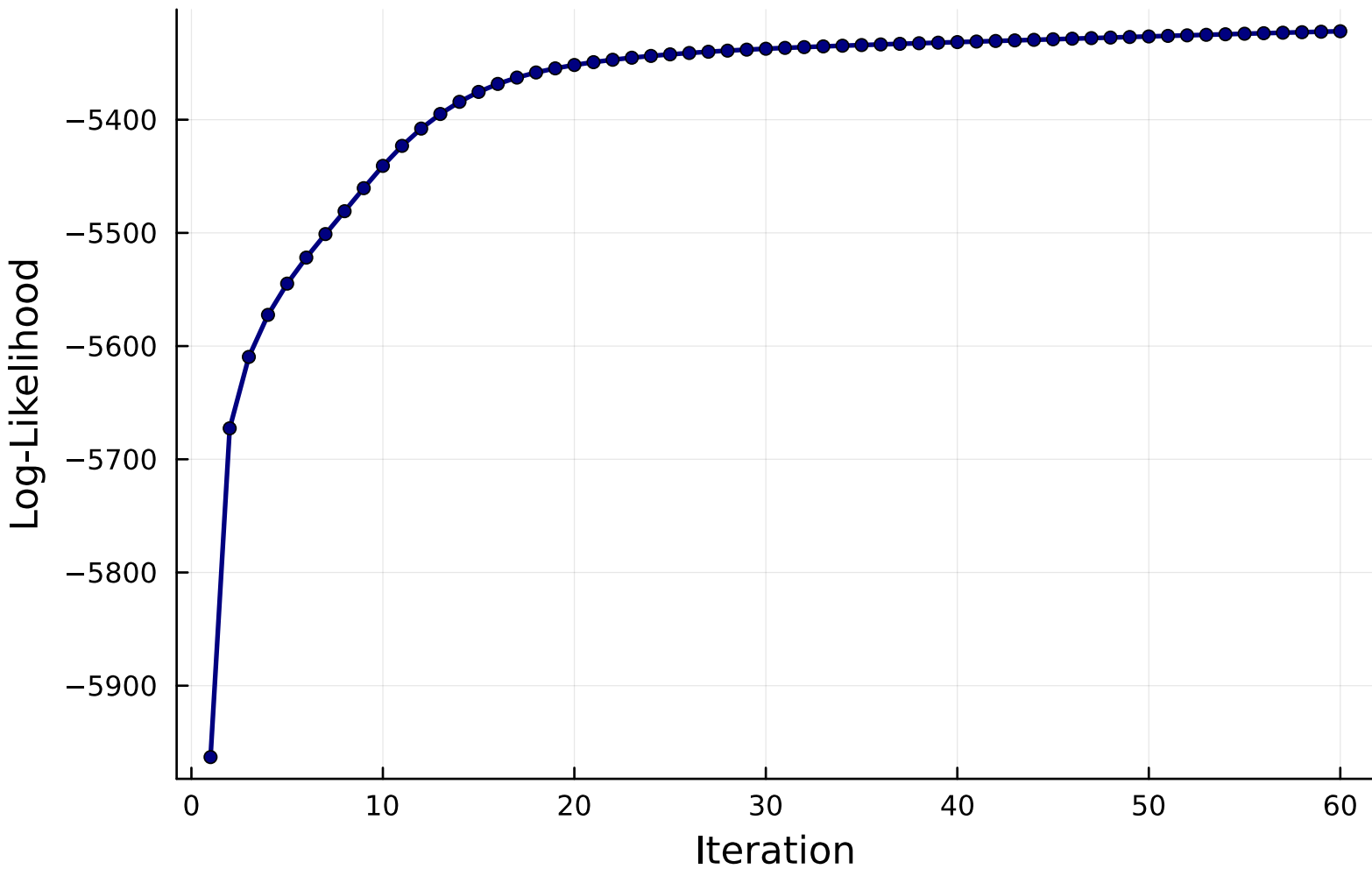
Baum-Welch Convergence (SPY, K=11)
