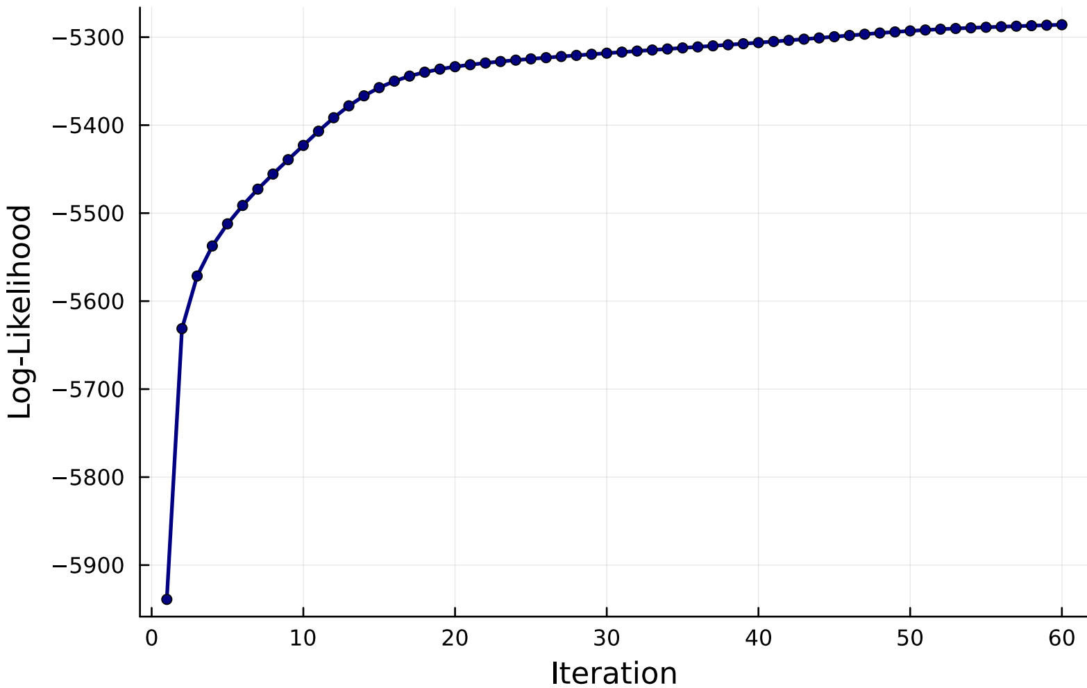
Baum-Welch Convergence (SPY, K=13)
