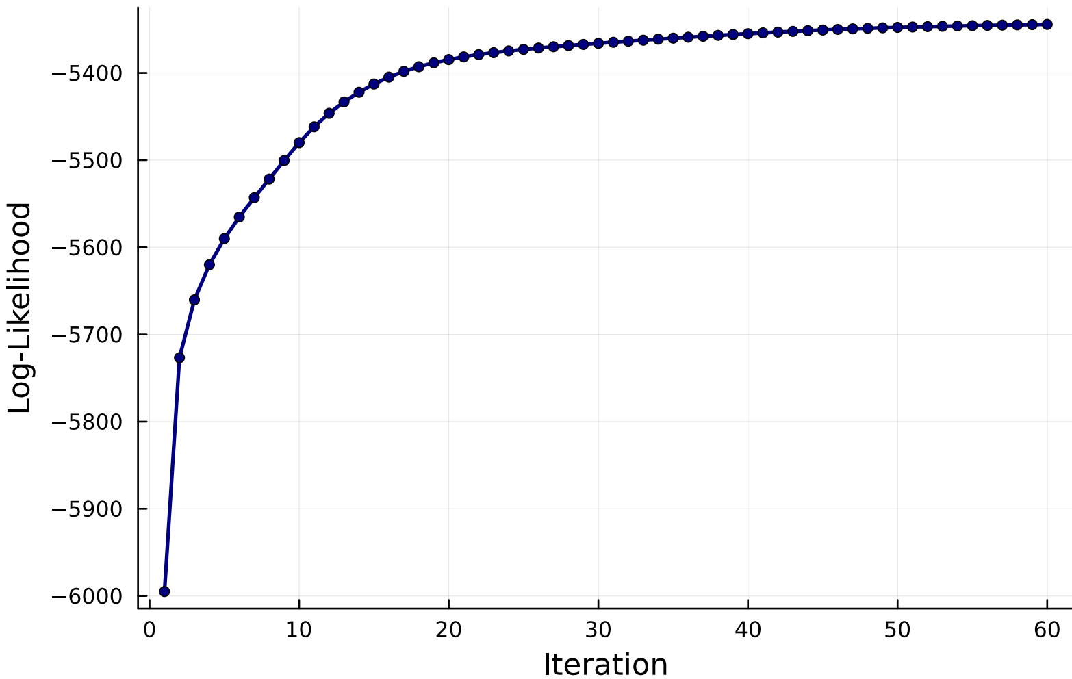
Baum-Welch Convergence (SPY, K=9)
