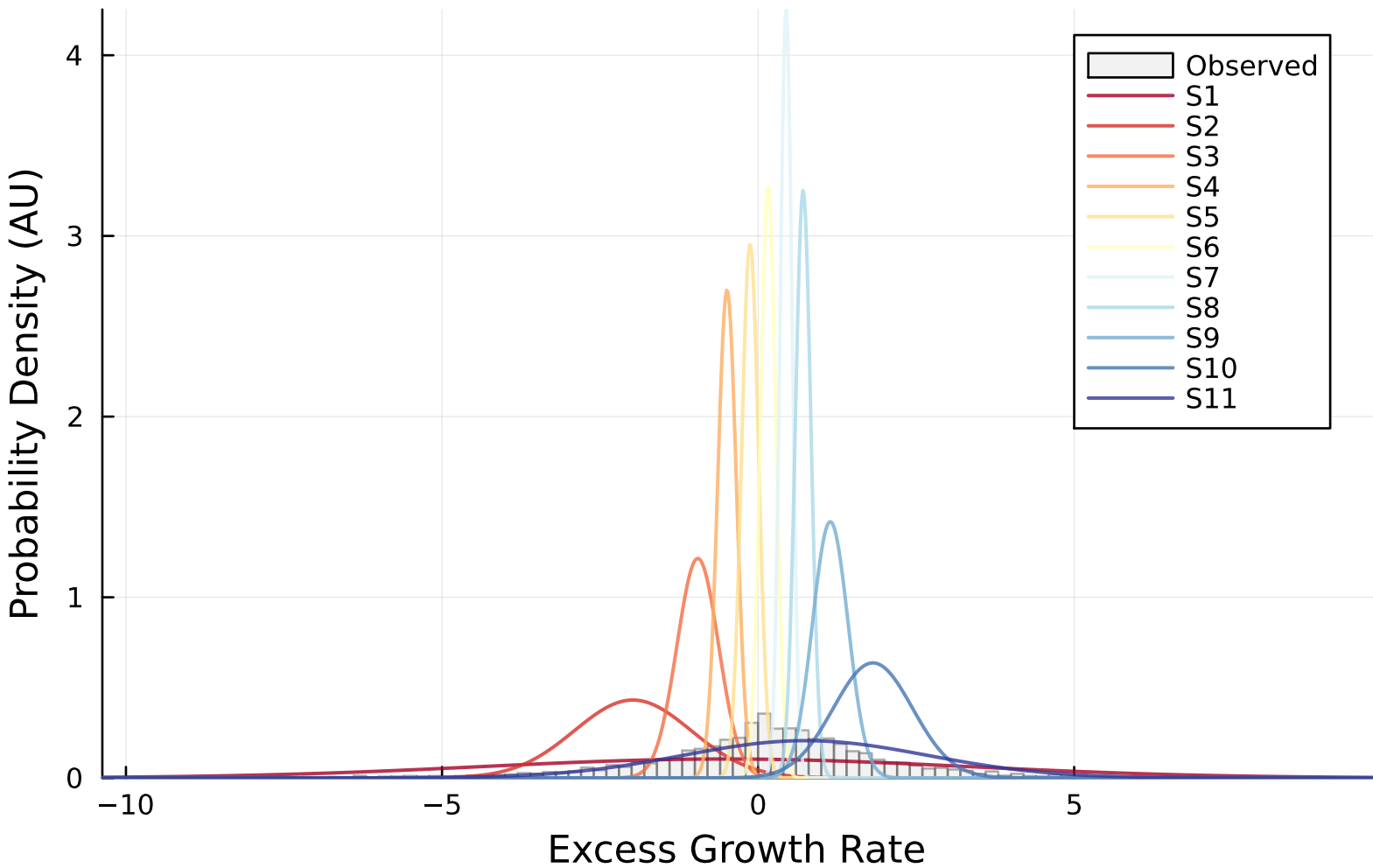
Emission Distributions (SPY, K=11)
