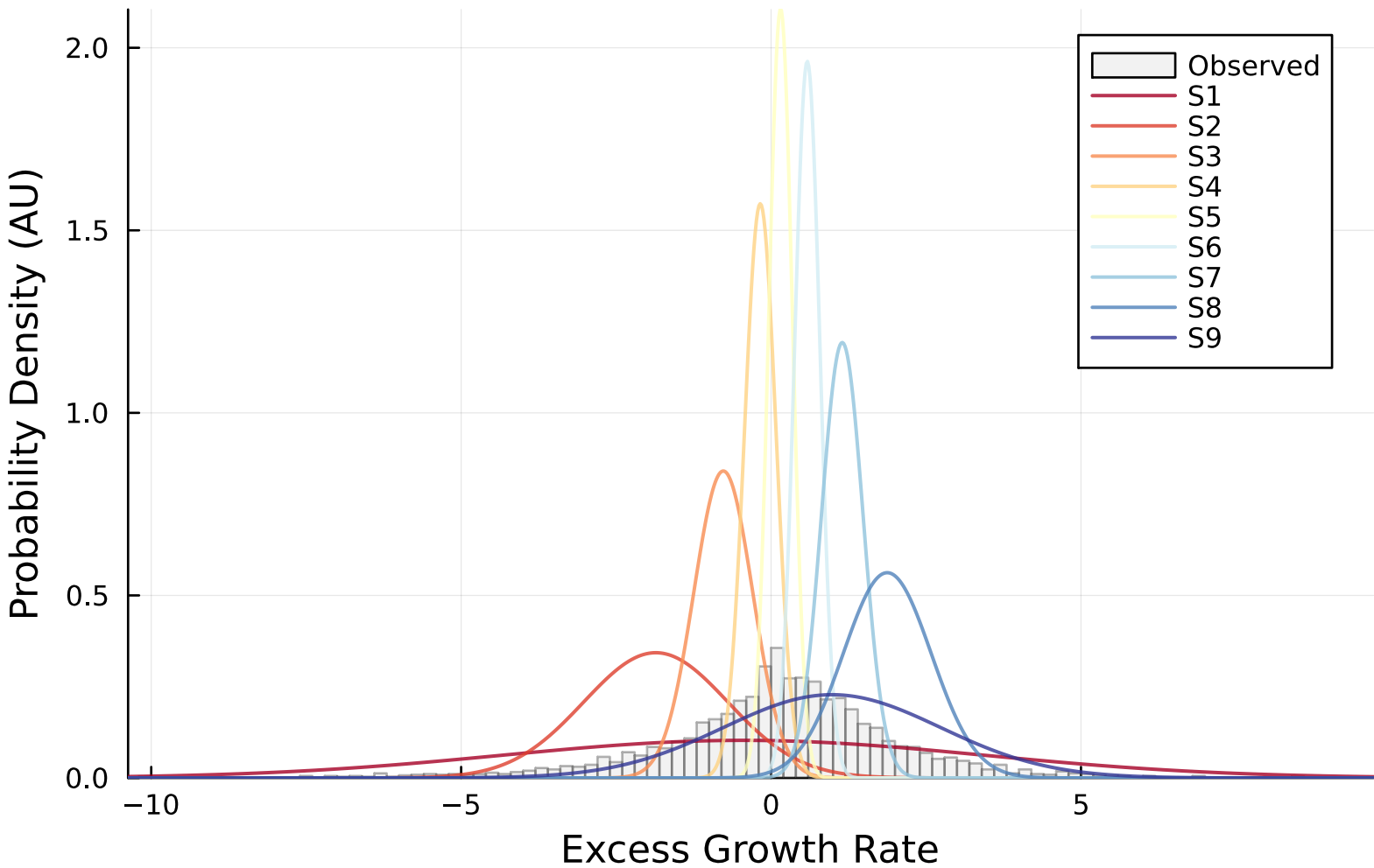
Emission Distributions (SPY, K=9)
