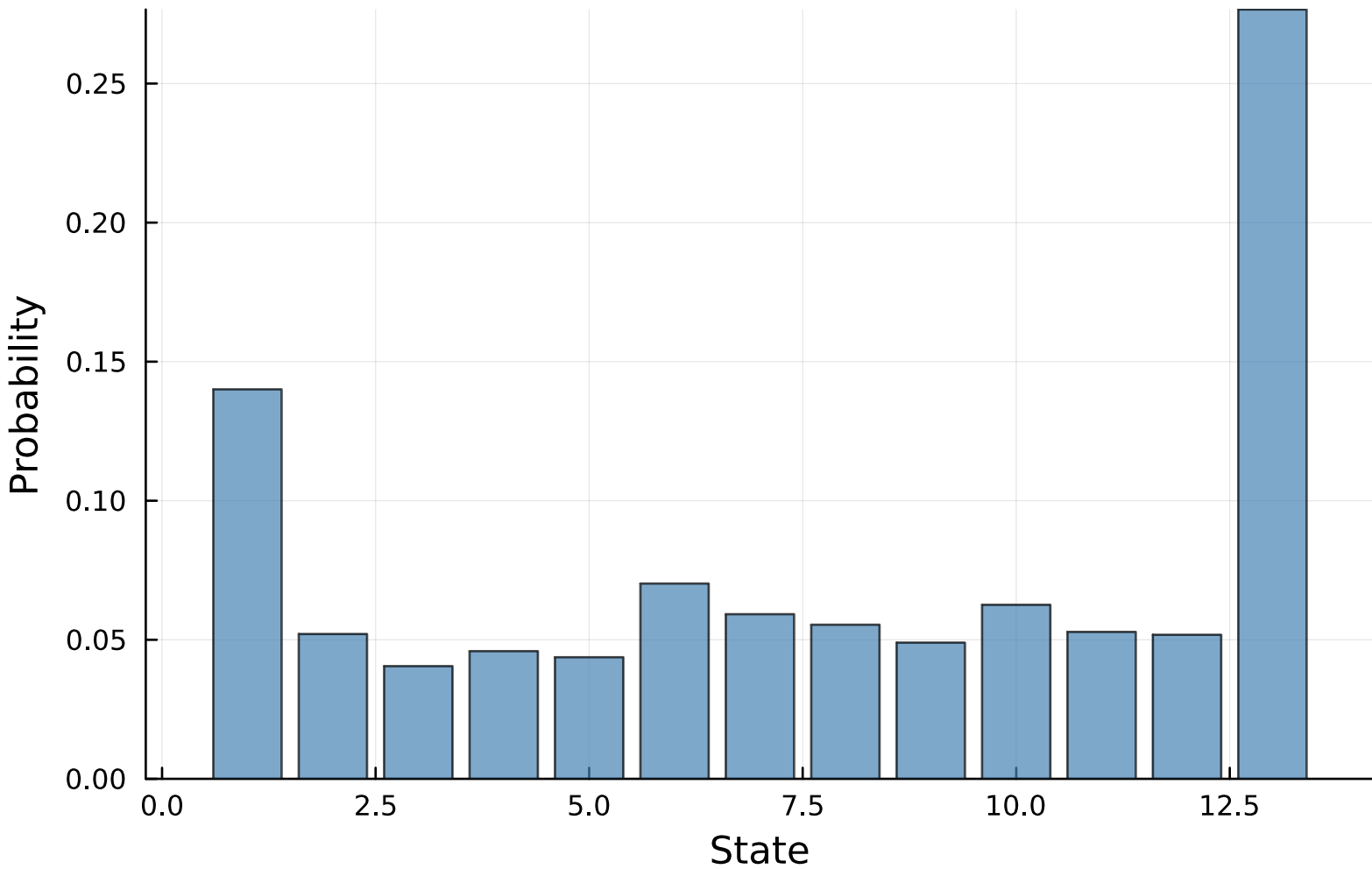
Stationary Distribution \pi — K=13
