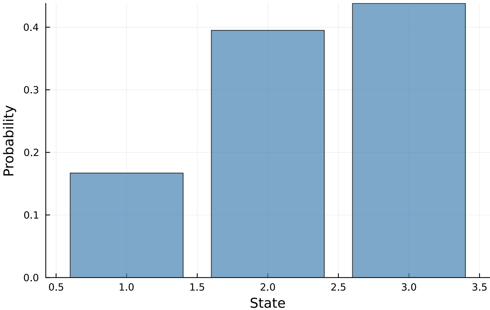
Stationary Distribution \pi — K=3
