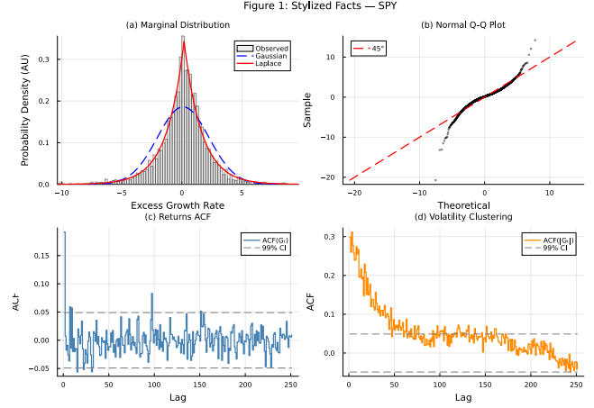
Figure 1: SPY stylized facts (IS, 2014-01-03 through 2024-01-03, T_{IS} = 2,516 ). Panel (a): marginal density with Gaussian and Laplace reference fits. Panel (b): normal Q-Q plot. Panel (c): ACF of G_t . Panel (d): ACF of |G_t| . Panels (a-b) evidence heavy tails; (c) evidences near-zero linear ACF; (d) evidences persistent volatility clustering.
