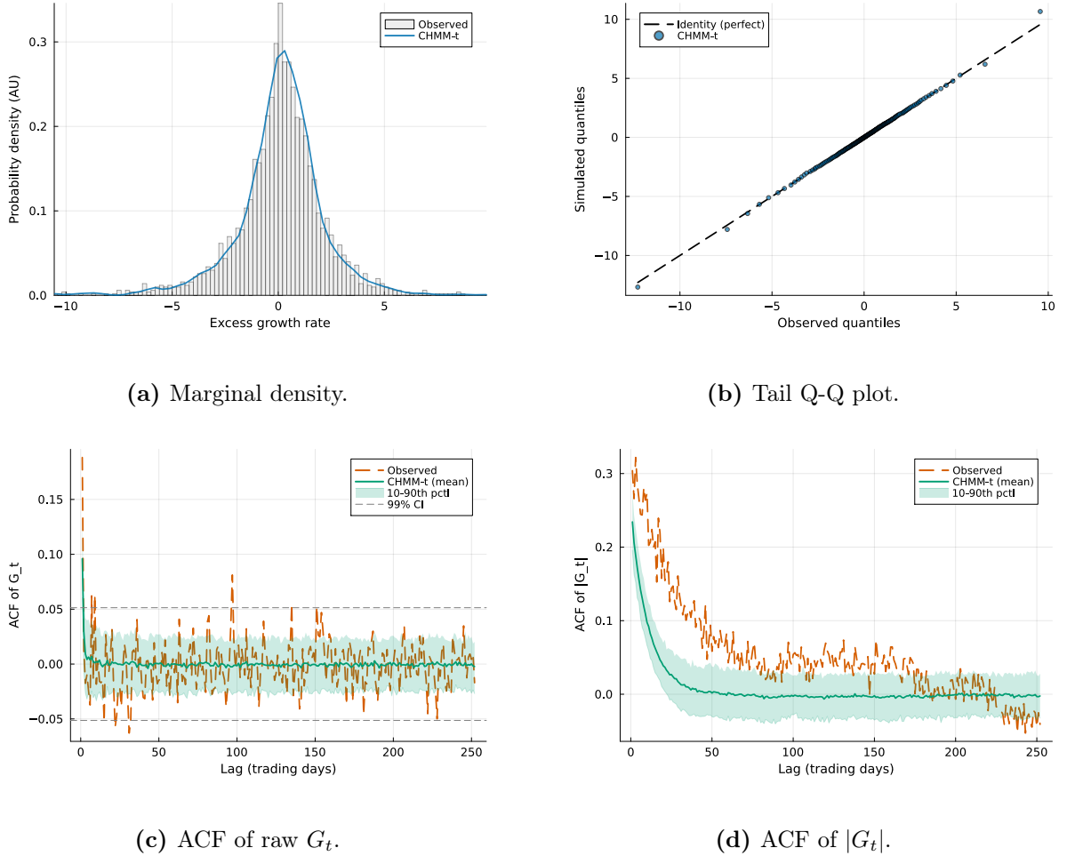
Figure 21. IS SPY model comparison at K = 18 for CHMM-t Student-t emissions (Pipeline A, 1,000 simulated paths). Panels show (a) marginal density with KS pass rate, (b) tail Q-Q plot, (c) ACF of raw G_t (linear autocorrelation, with the 99% Bartlett band), and (d) ACF of |G_t| (volatility clustering). The CHMM-N counterpart is Figure 4; the CHMM-L and CHMM-GED counterparts are Figures 22 and 23.
