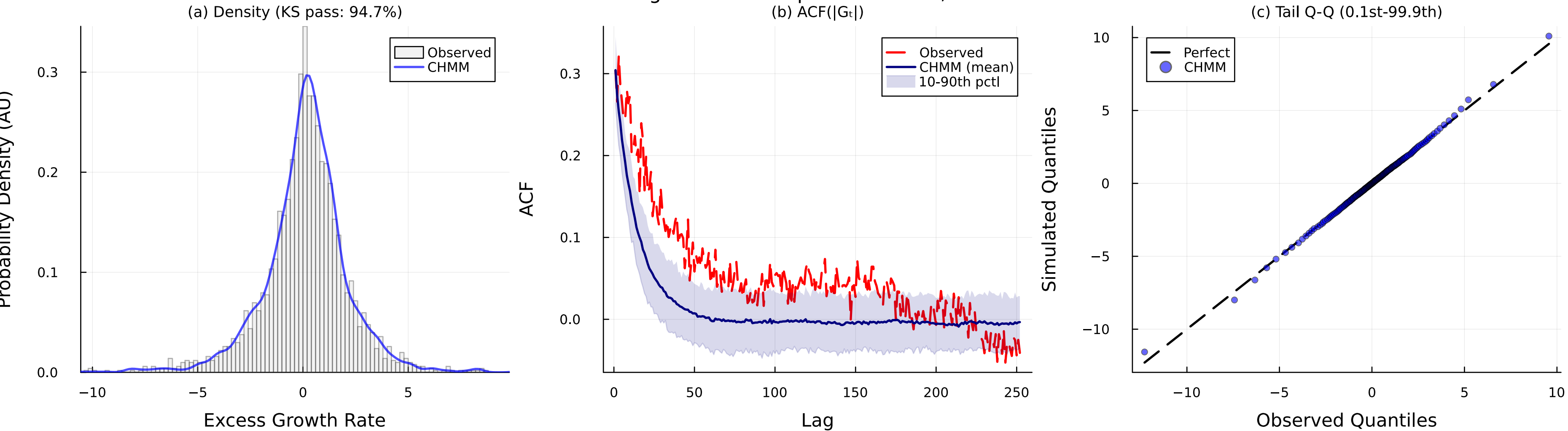
Figure 3: IS Comparison — SPY, K=15
