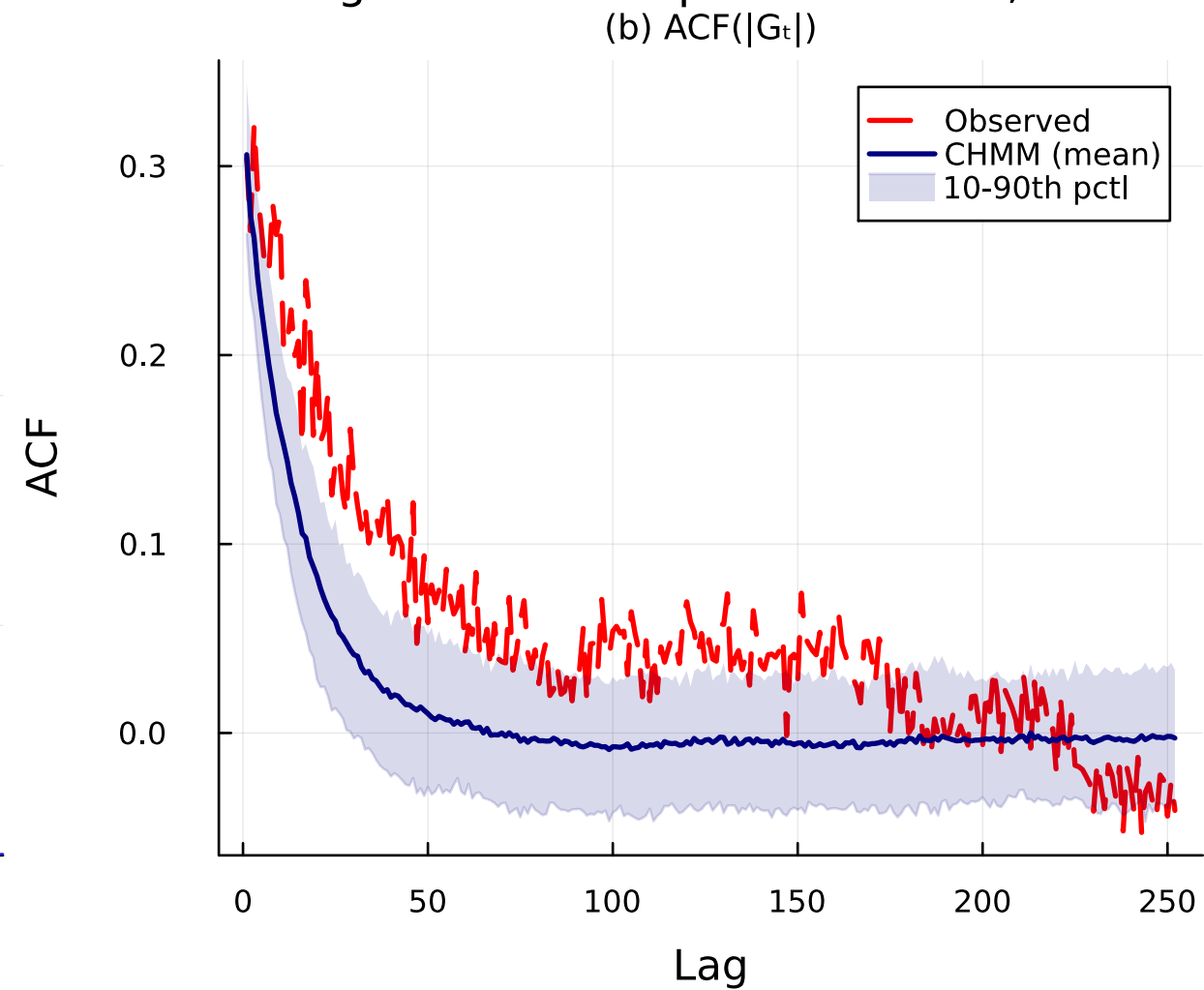
Figure 3: IS Comparison — SPY, K=9
