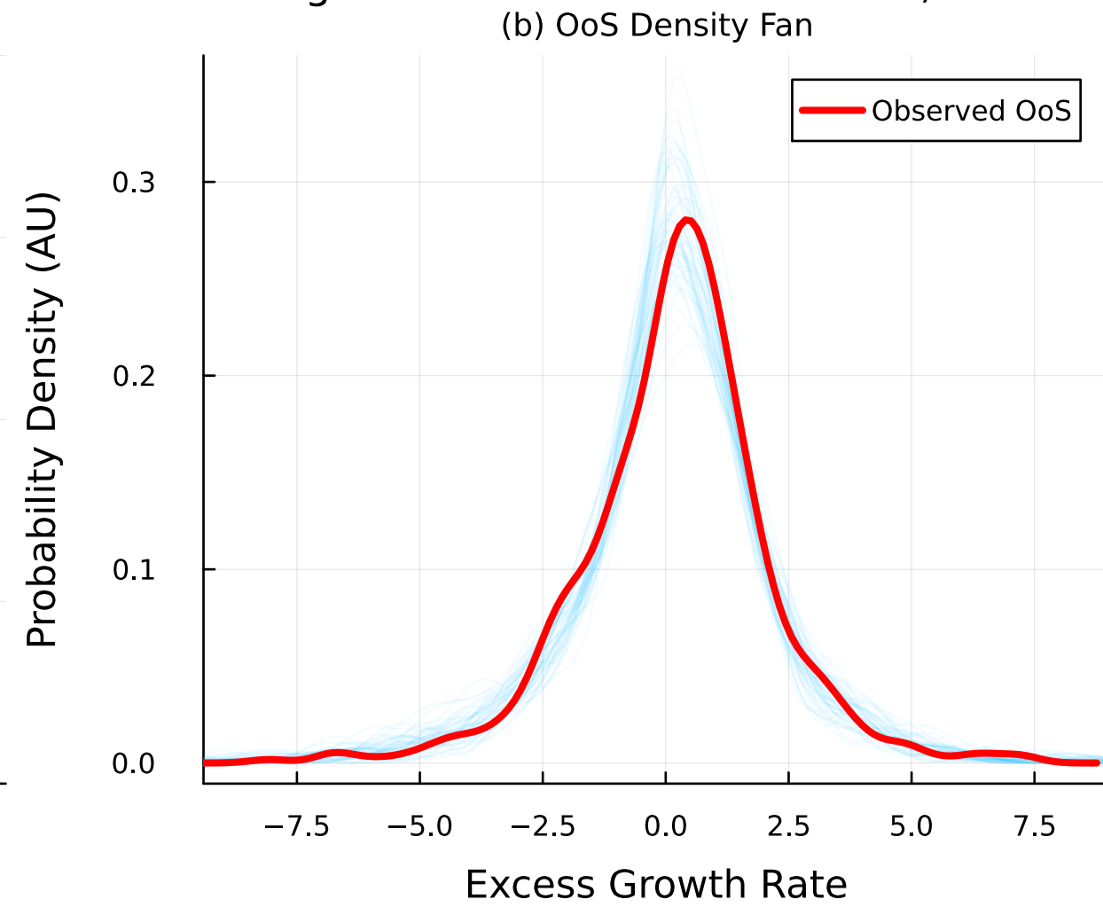
Figure 4: OoS Validation — SPY, K=18
