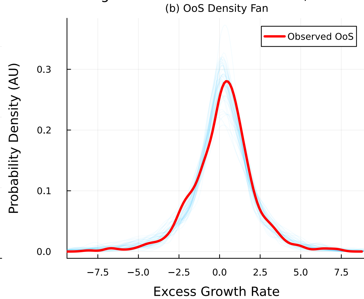
Figure 4: OoS Validation — SPY, K=21
