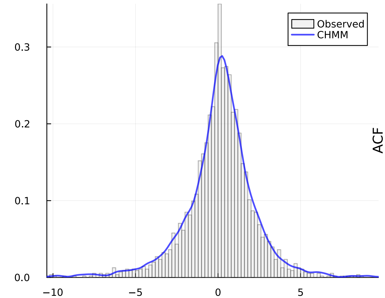
(a) Density (KS pass: 94.5%)
