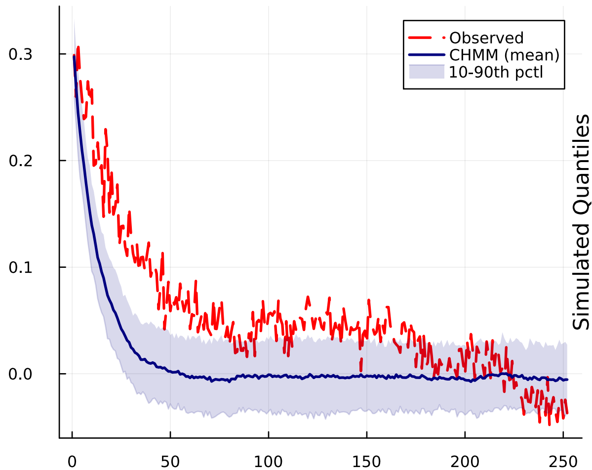
(b) ACF( |G_t| )
