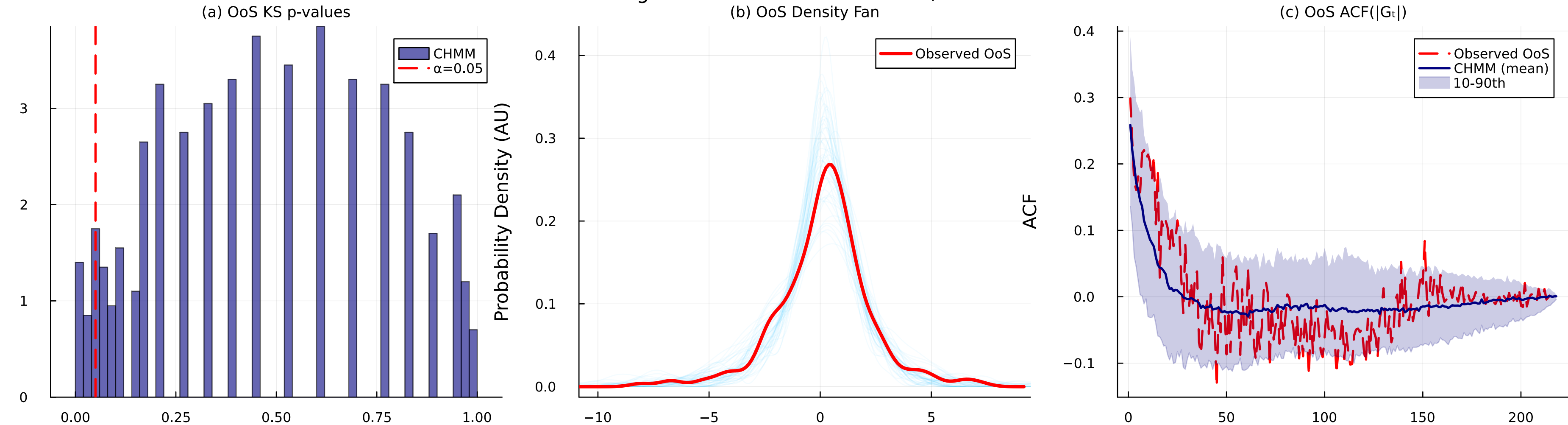
Figure 4: OoS Validation — SPY, K=12
