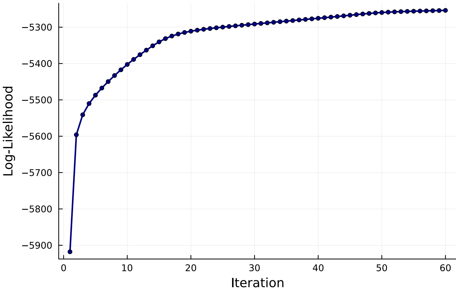
Baum-Welch Convergence (SPY, K=15)
