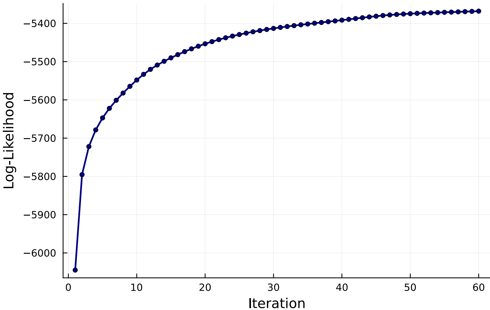
Baum-Welch Convergence (SPY, K=6)
