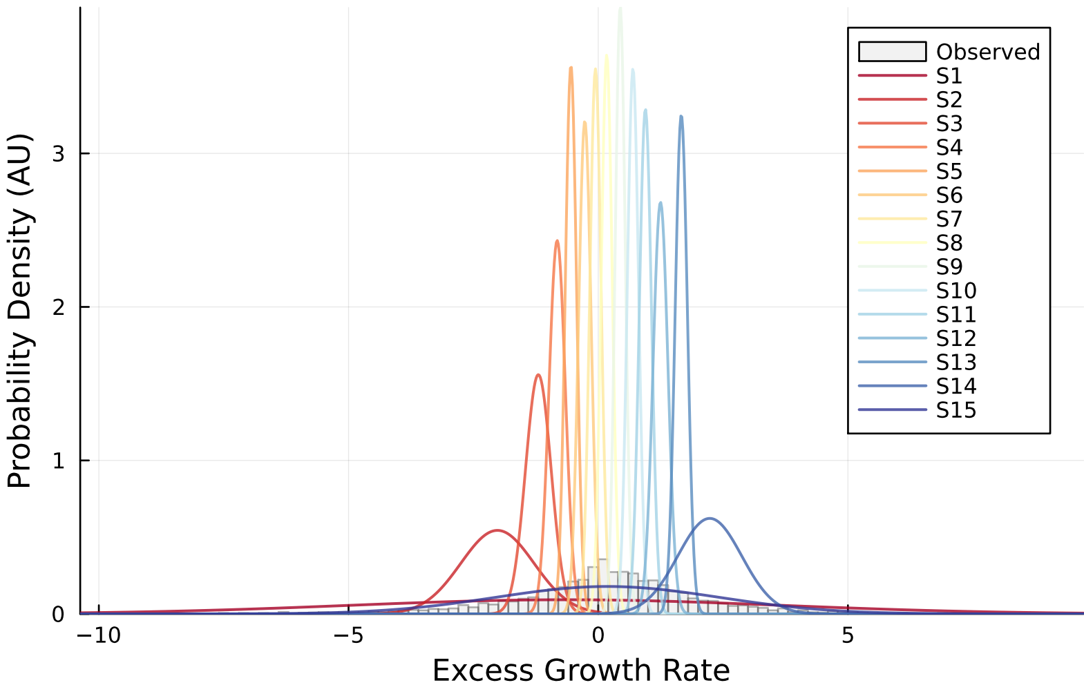
Emission Distributions (SPY, K=15)
