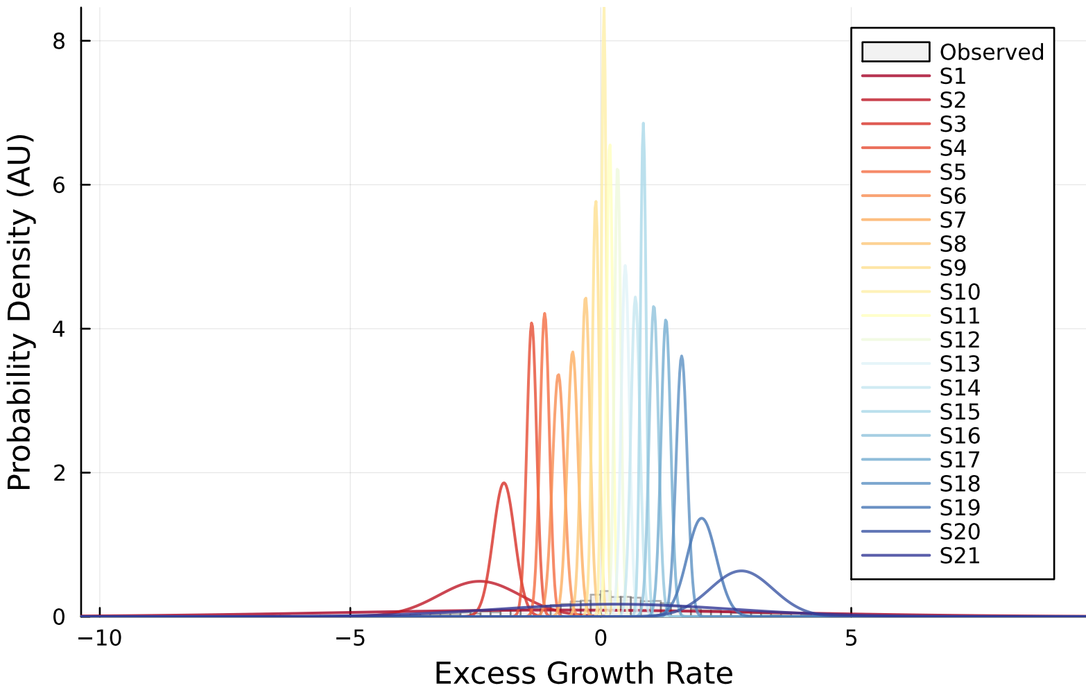
Emission Distributions (SPY, K=21)
