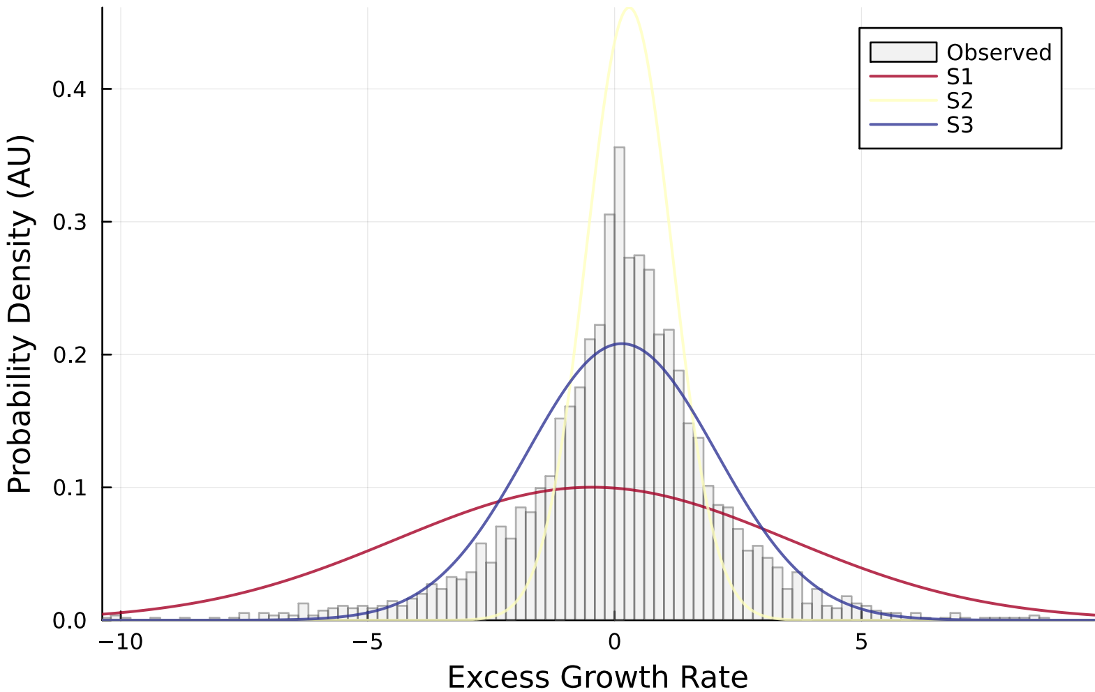
Emission Distributions (SPY, K=3)
