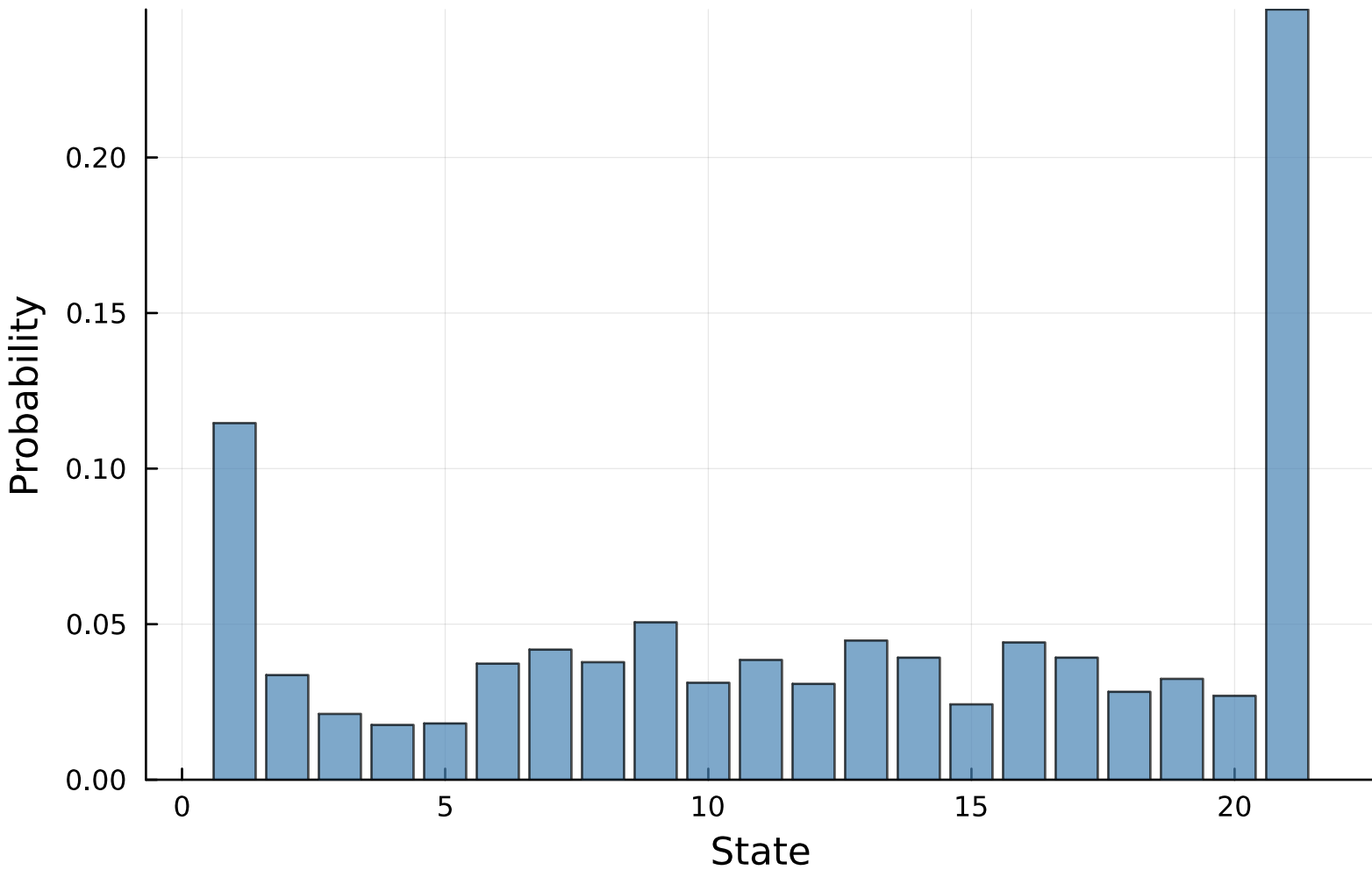
Stationary Distribution \pi — K=21
