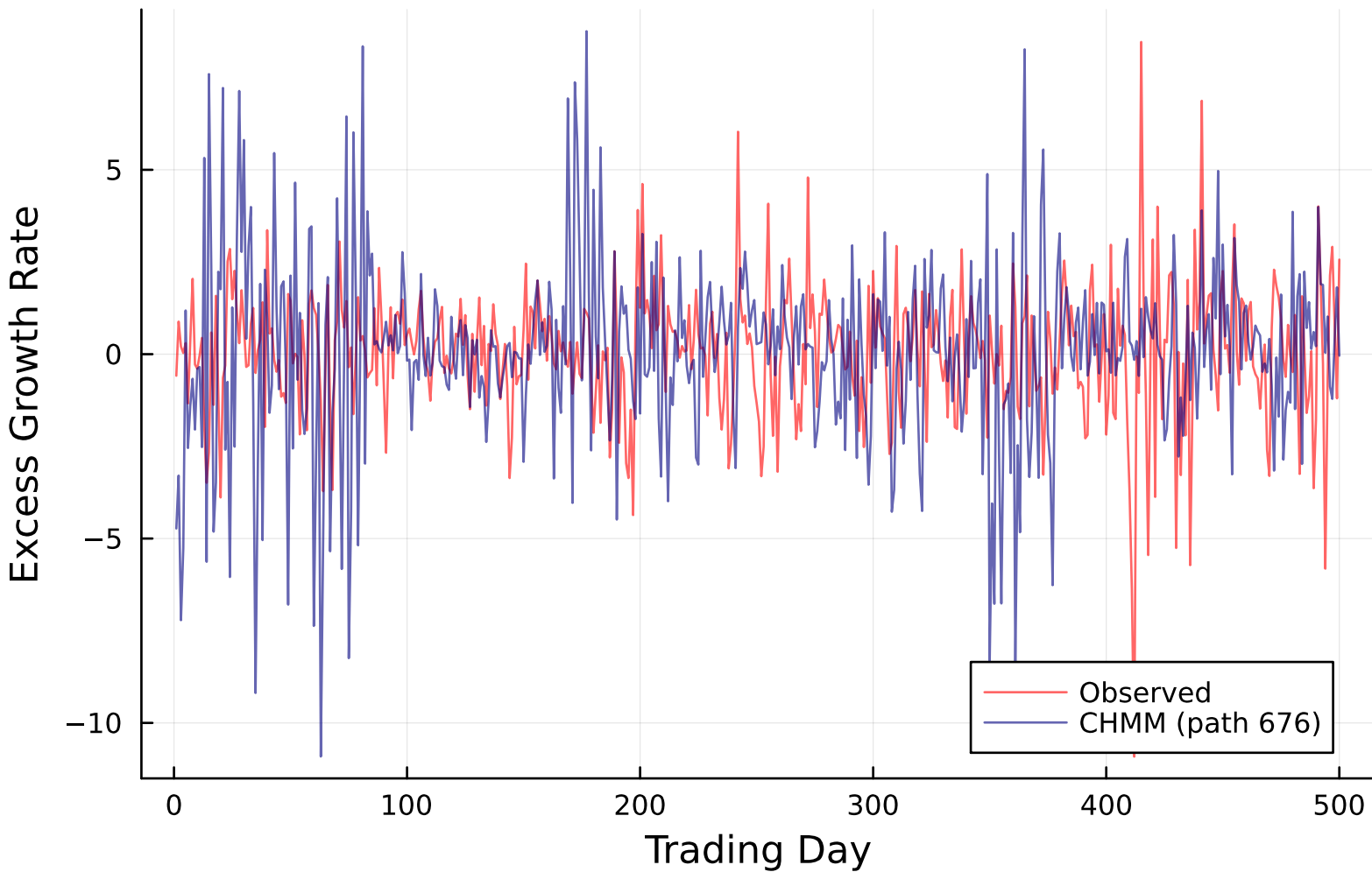
Return Trajectory (first 500 steps) — K=12
