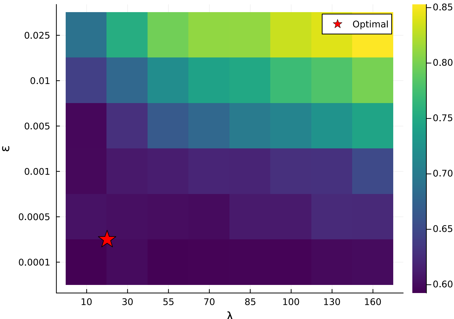
Grid Search J(\epsilon, \lambda) — K=11
