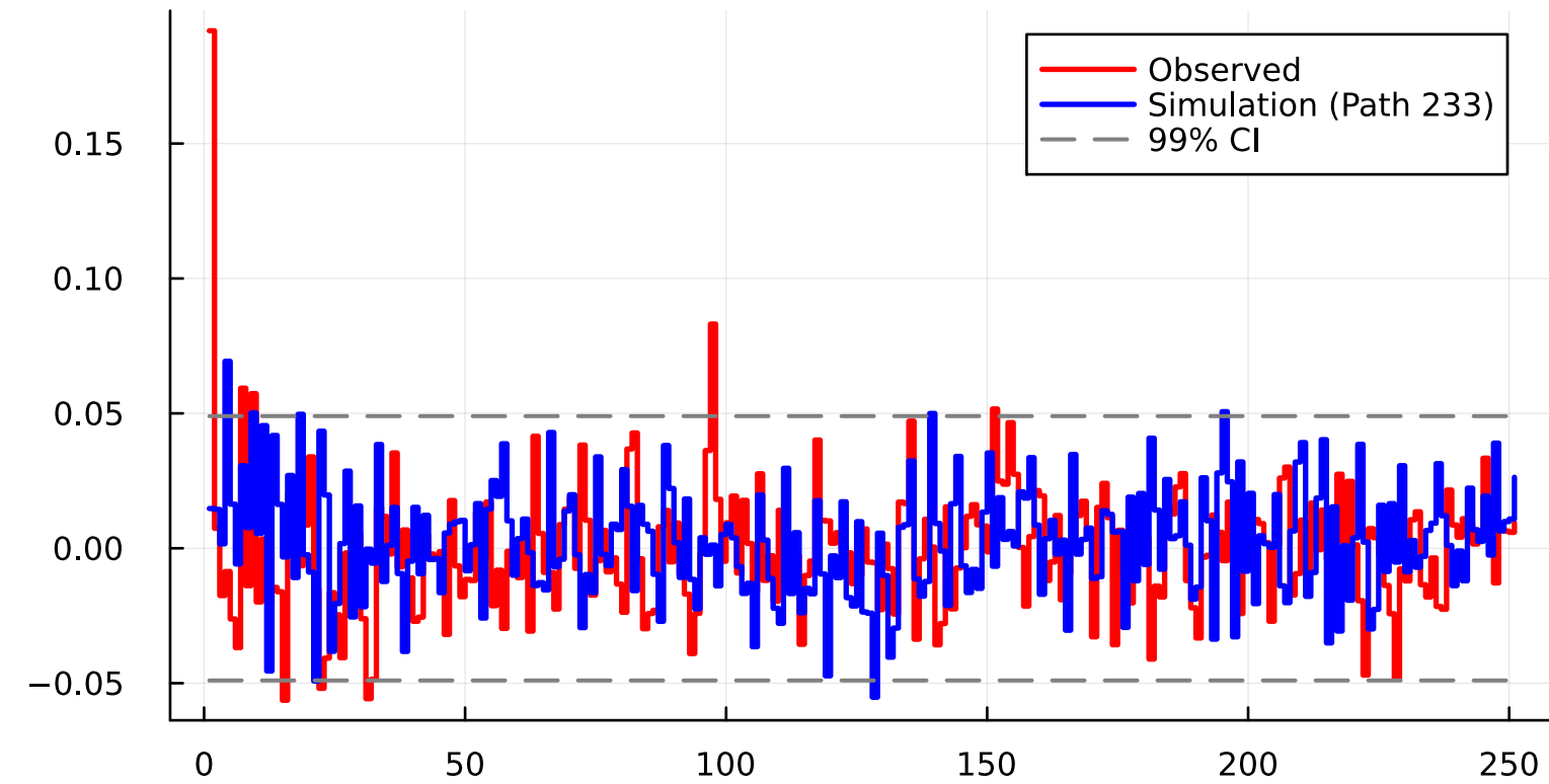
Lag (trading day) |Returns| ACF — WJ, K=6
