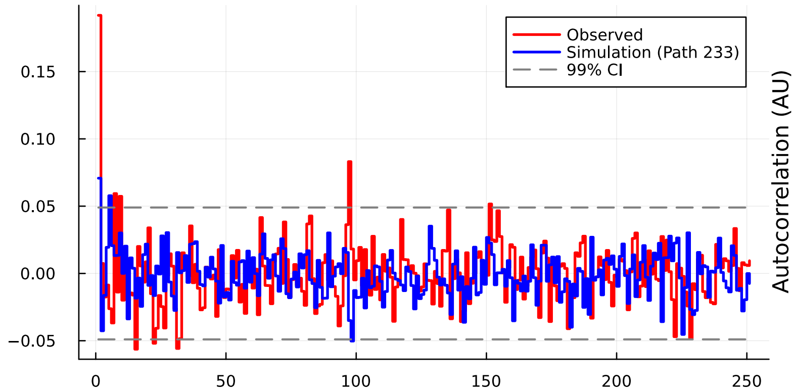
Lag (trading day) |Returns| ACF — NJ, K=6
