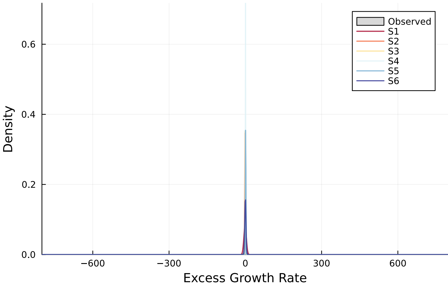
Emission Distributions (SPY, K=6)
