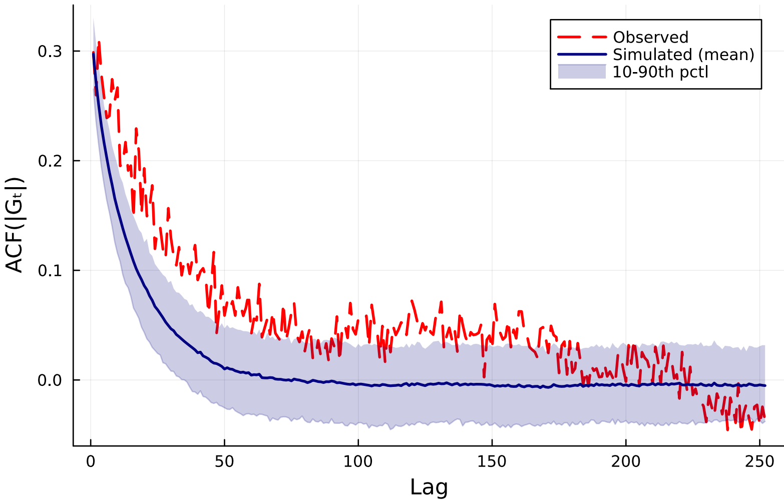
ACF( |G_t| ) at Optimal — K=9 ( \varepsilon=0.0001 , \lambda=55 )
