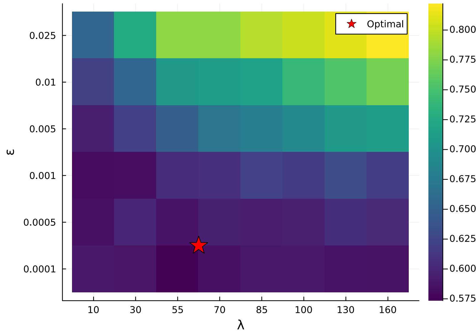
Grid Search J(\epsilon, \lambda) — K=9
